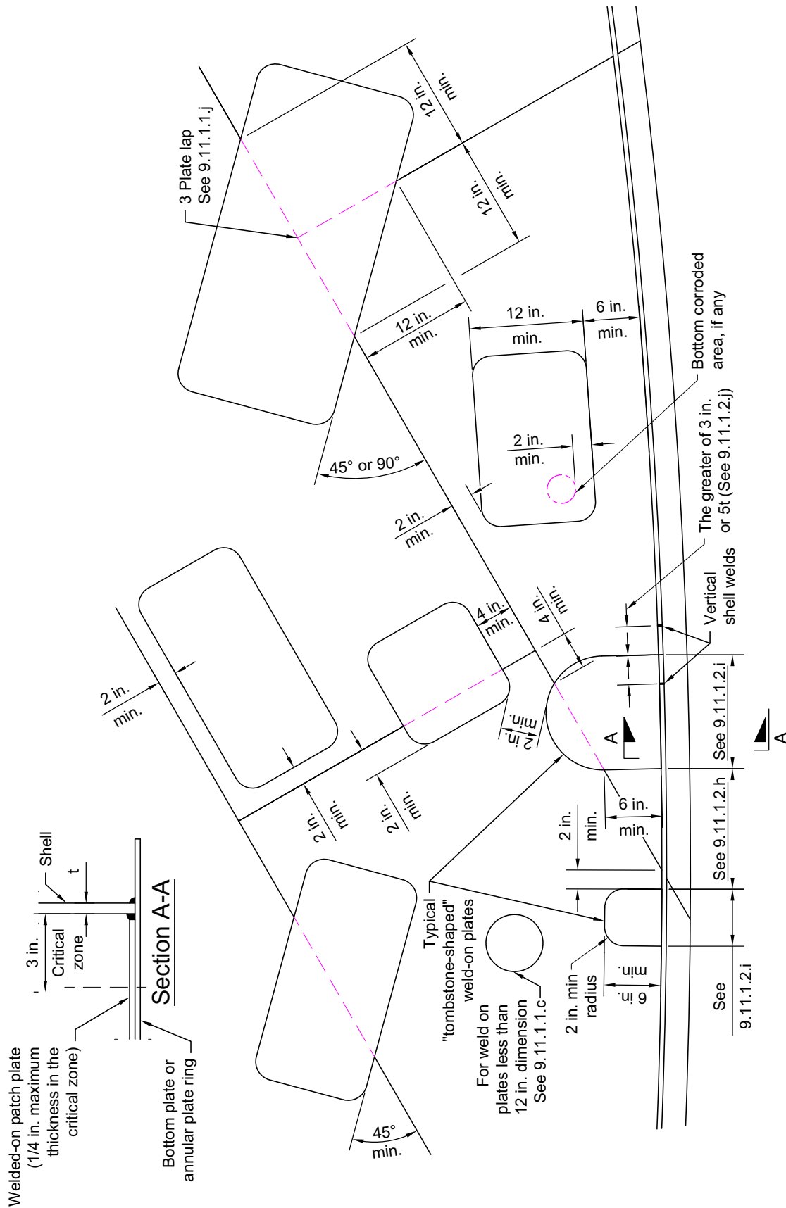
Figure 9.13b—Typical Welded-on Patch Plates on Tank Bottom Plates, in USC Units
