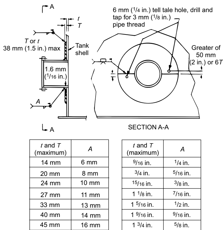
Figure 9.7—Typical Details for Addition of Reinforcing Plate to Existing Shell Penetration
