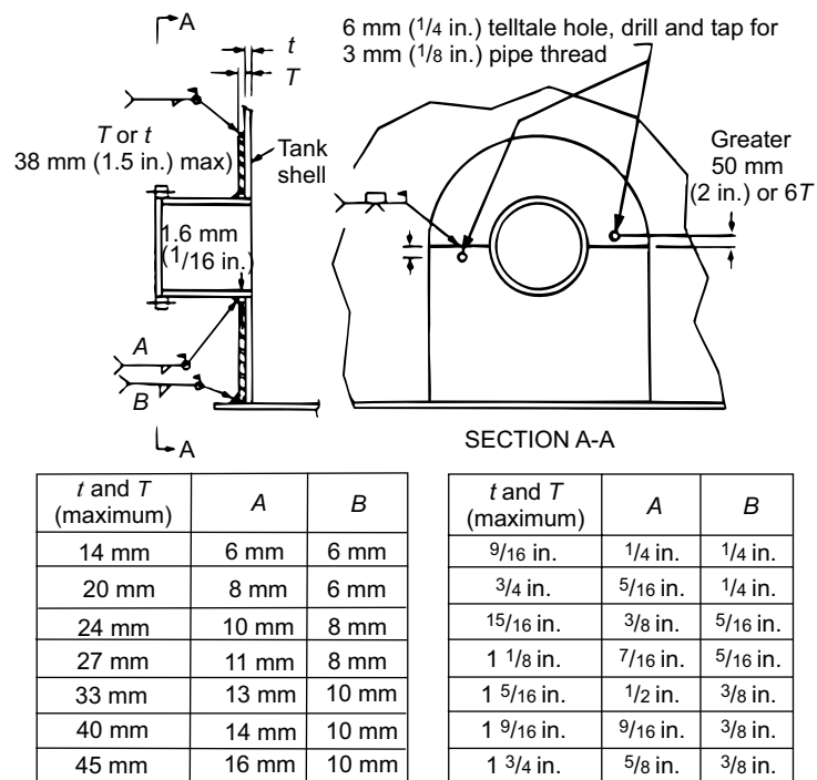
Figure 9.7—Typical Details for Addition of Reinforcing Plate to Existing Shell Penetration
